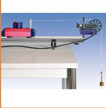
Inclined plane + Trolley
